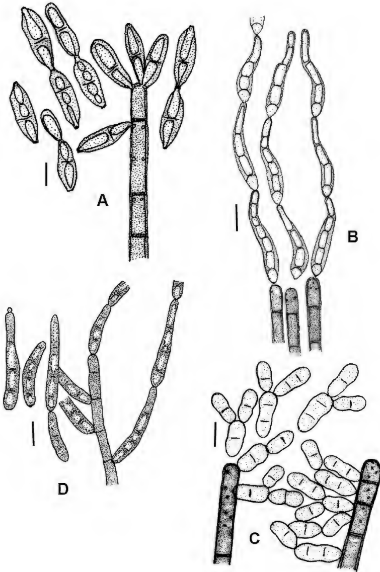
FIG. 1. Ellismarsporium species: conidiogenous cells and conidia. A. E. hypselodelphyos (Ellis 1961); B. E. catenatum (Matsushima 1975); C. E. parvum (Castañeda-Ruiz & Kendrick 1991); D. E. pinarense (Castañeda-Ruiz 1985). Scale bars: A, C, D = 10 \mu m; B = 20 \mu m. Redrawn by R.F. Castañeda-Ruiz.
