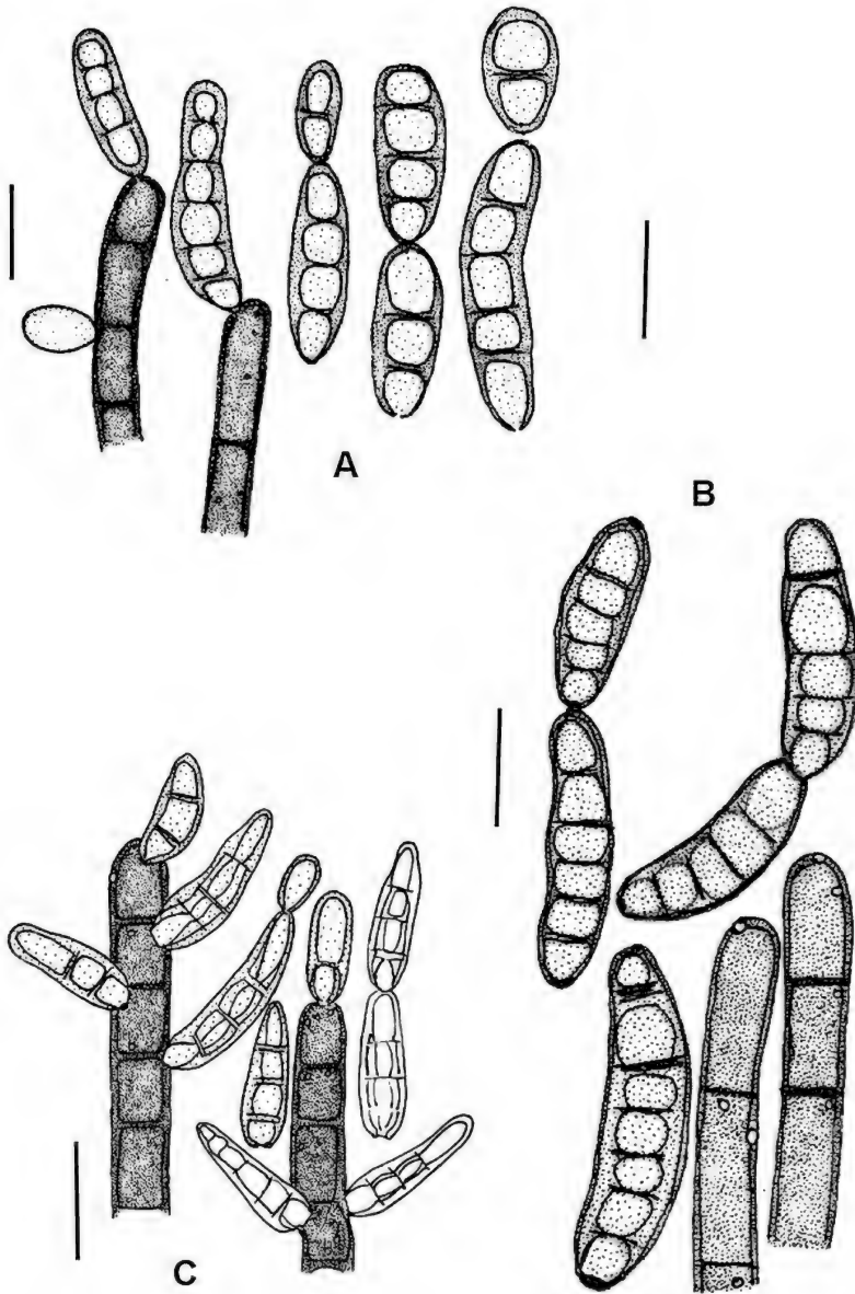
FIG. 2. Ellismarsporium species: conidiogenous cells and conidia. A. E. senseletii (Bhat & Sutton 1985); B. E. simpliphorum (Matsushima 1993); C. E. zombaense (Sutton 1993). Scale bars: A, B = 10 \mu m; C = 20 \mu m. Redrawn by R.F. Castañeda-Ruiz.
