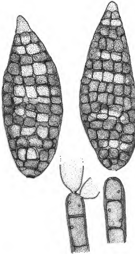
FIG. 3. Stanhughesiella dictyoseptata : conidiogenous cells and conidia (Hughes 1980). Scale bar = 10 \mu m. Redrawn by R.F. Castañeda-Ruiz.
